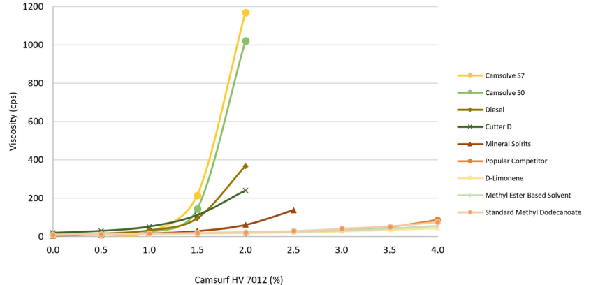
VISCOSIFYING PROPERTIES OF HV-7012 WITH DIFFERENT SOLVENTS (Brookfield RVF Viscometer, #2 spindle, 21°C, 20 rpm)
